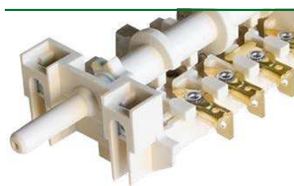
Plastic shaft
